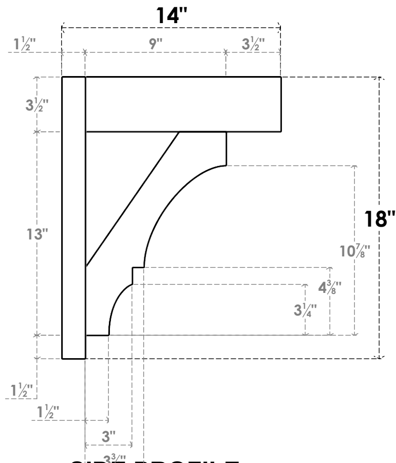
SIDE PROFILE
